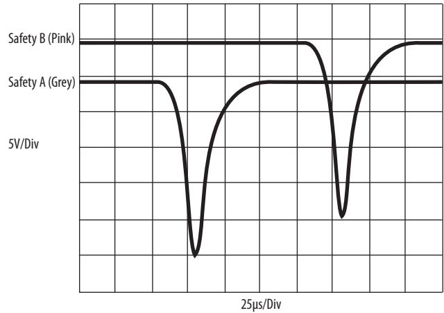
Figure 15 - Output Test Pulses
