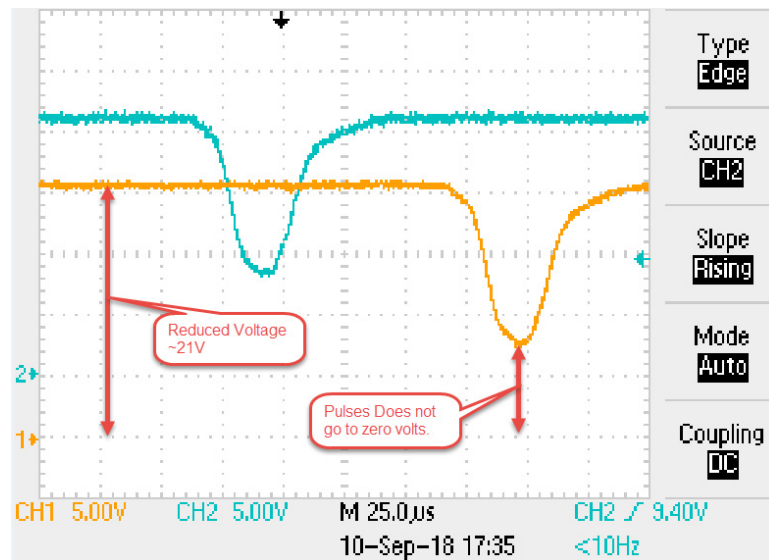
Figure 41 - Effect of 300 ohms of Wire Resistance Going Into a GSR-SI Safety Relay
