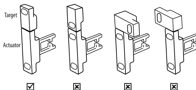
Figure 2 - Target/Actuator Mounting
