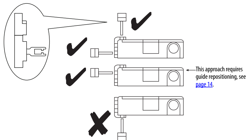
Figure 3 - Allowable Approach Direction
