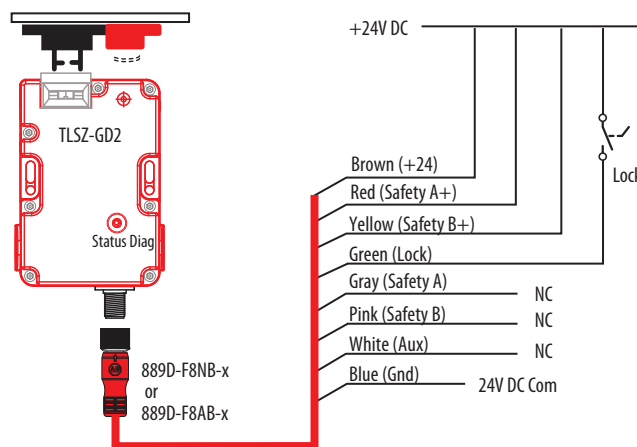
Figure 16 - Commissioning Wiring
