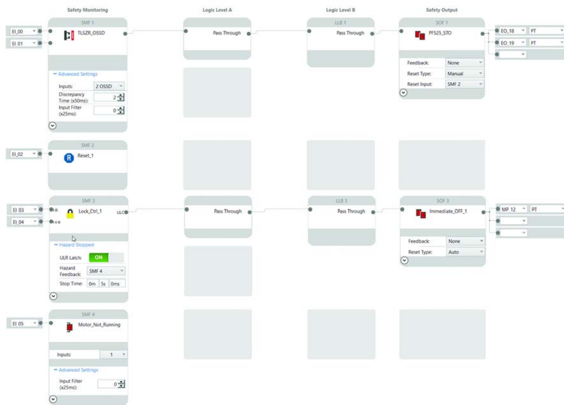
Figure 22 - CR30 Configuration in CCW
