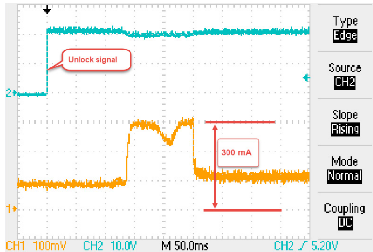
Figure 44 - In-rush Current on the Power Supply at the Switch
