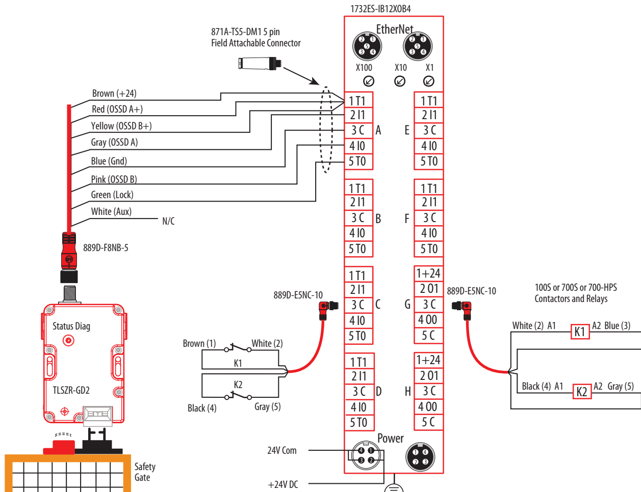
Figure 30 - ArmorBlock Schematic
