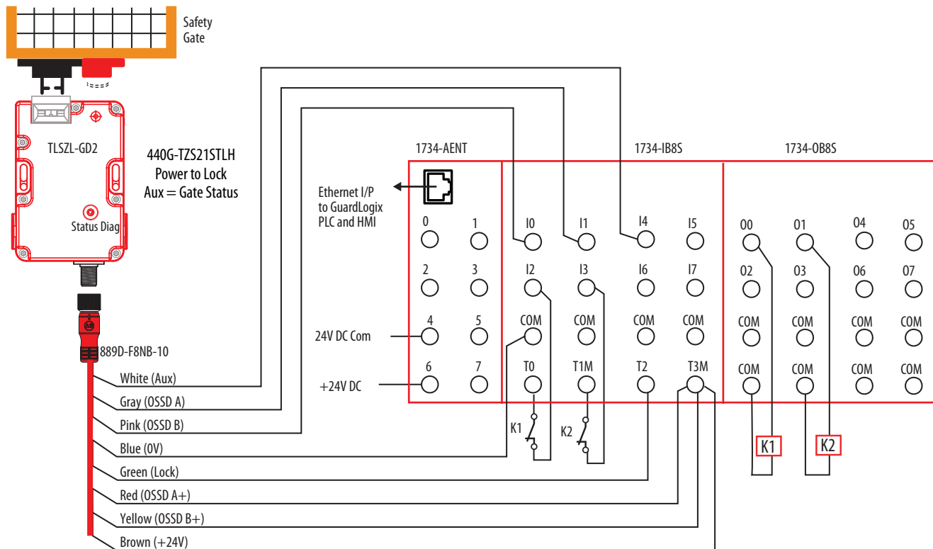
Figure 23 - 1734 and TLSZL Schematic
