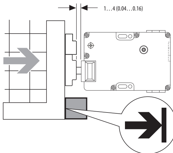
Figure 10 - Clearance and Insertion Distance
