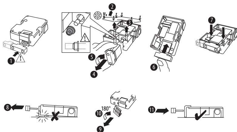
Figure 8 - Guide Repositioning
