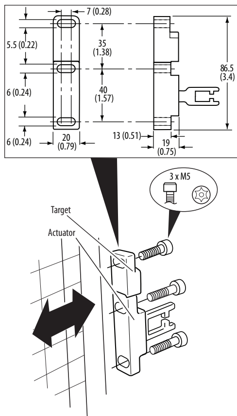
Figure 13 - Actuator/Target Mounting Dimensions [mm (in.)]
