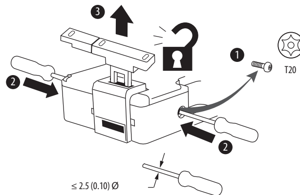
Figure 6 - Manual Release
