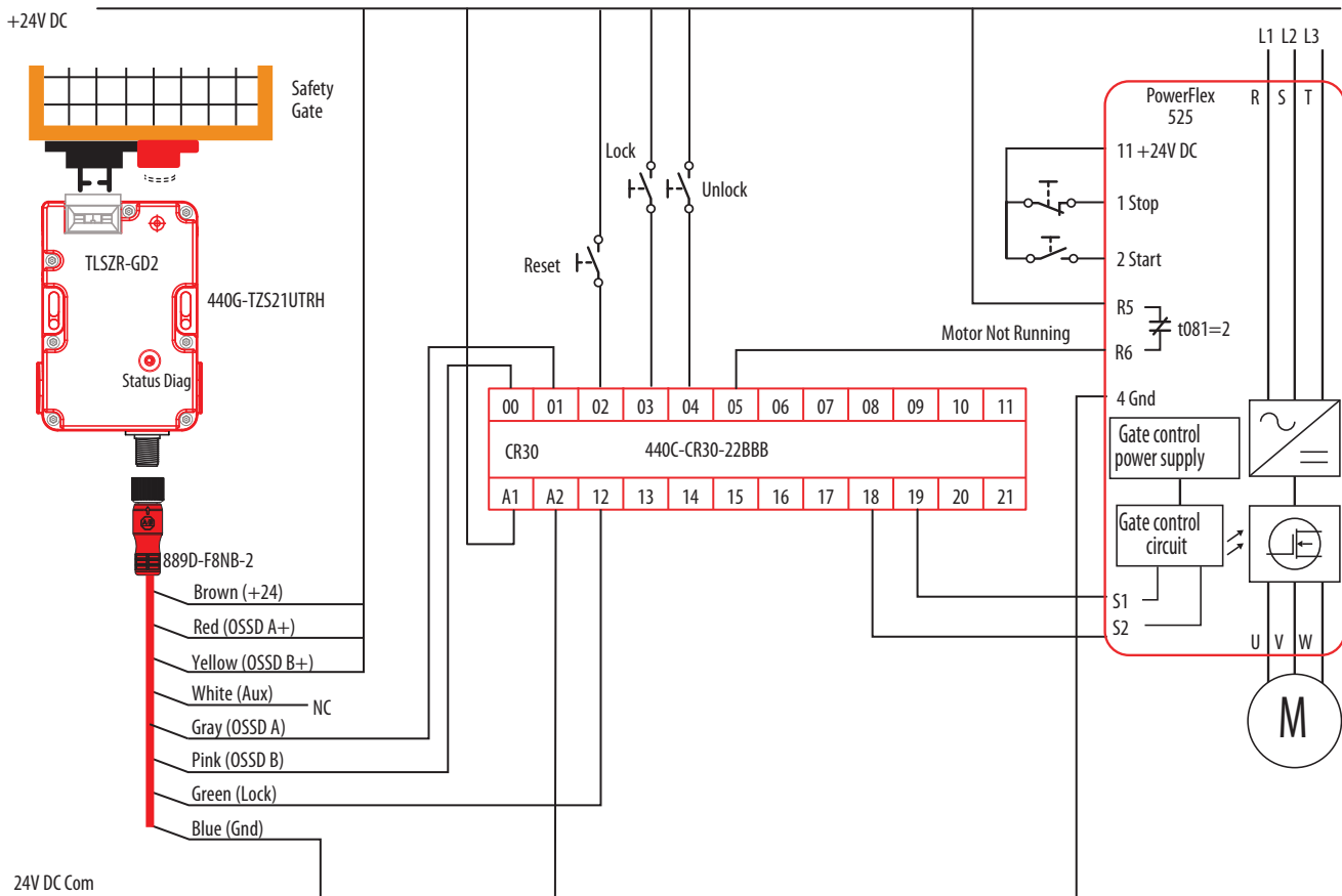
Figure 21 - CR30 Schematic
