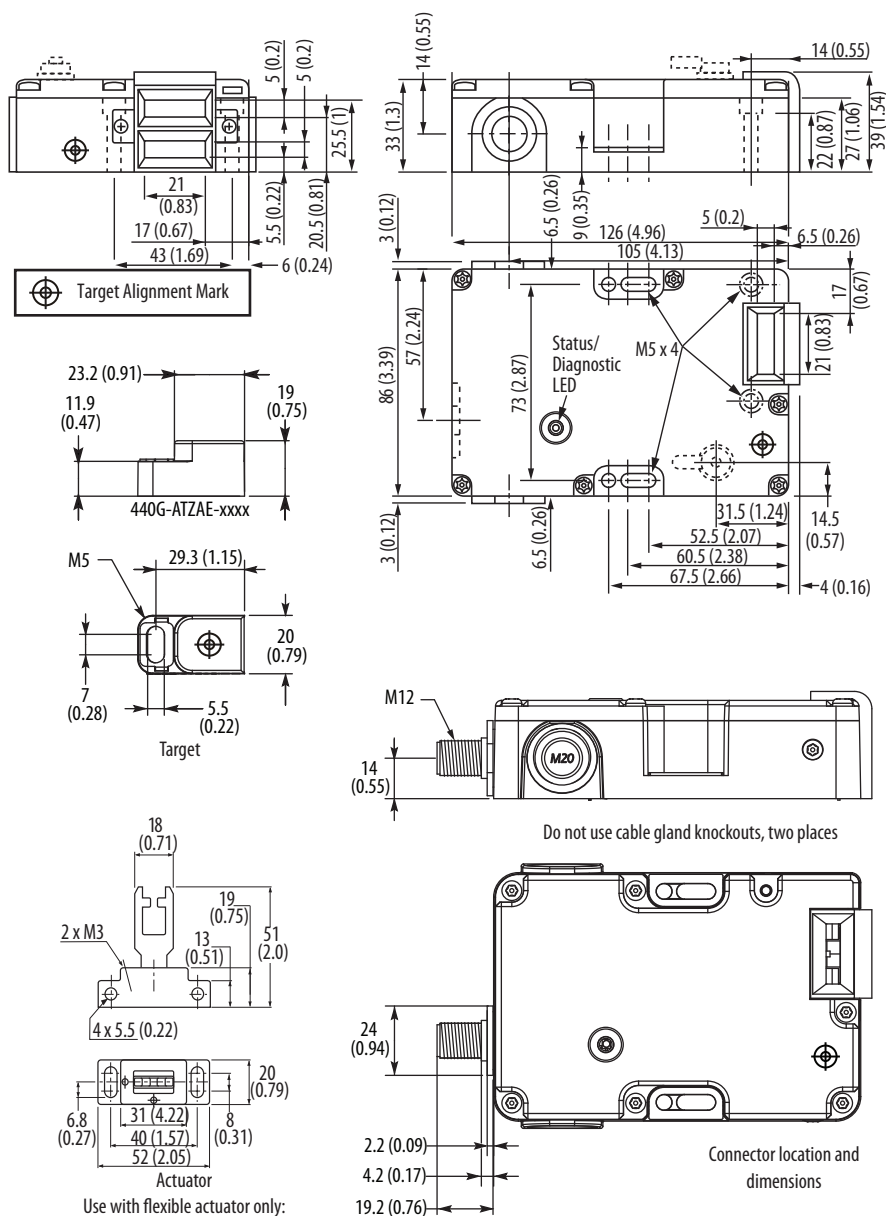
Figure 12 - Dimensions [mm (in.)]
