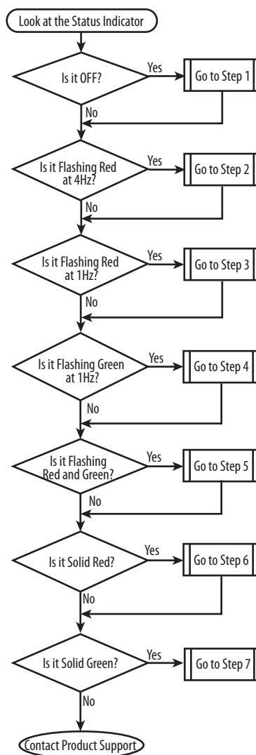
Figure 36 - Troubleshooting Flow Diagram
