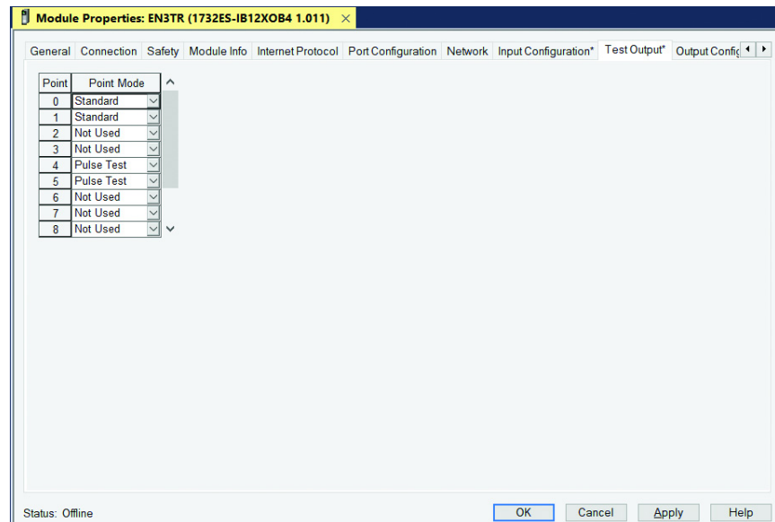
Figure 33 - Module Properties – Test Output
